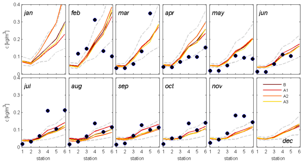
Fig. 5 Monthly averaged observed surface sediment concentration (black dots, February through November) and model realisations in 2012 at stations S1 to S6 (in \text{kg/m}^3 ). The colours refer to the model realisation, and the grey dashed line is the standard deviation of the
