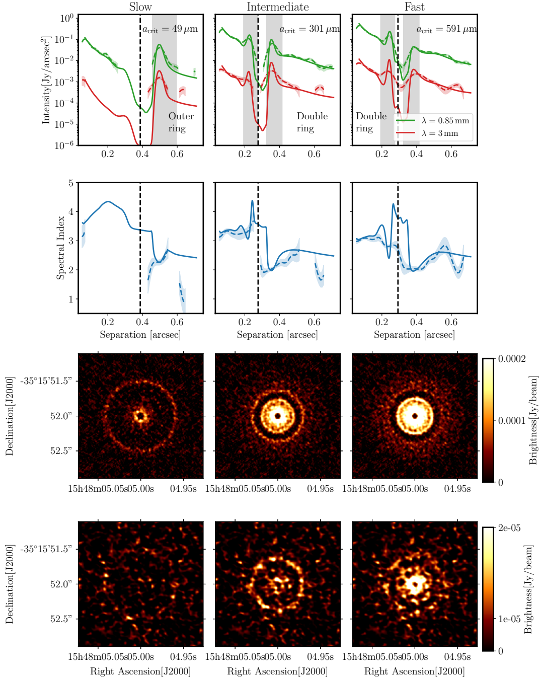
Figure 2. The same as Figure 1 for a_{\text{max}} = 1 cm. With the presence of larger grains, the intensity profile of the ‘Fast’ simulation shows two maxima—i.e. this simulation produces structures similar to the ‘intermediate’ simulation.
