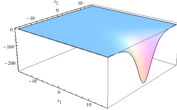
FIGURE 6. Graph of K_4 .
