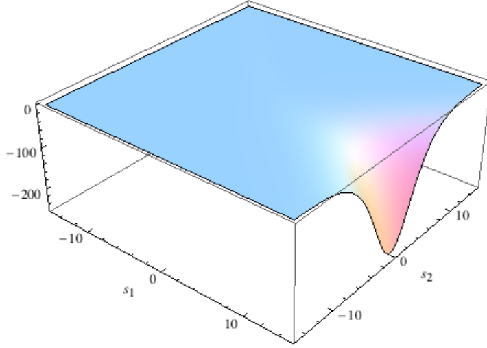
FIGURE 8. Graph of K_5 .
