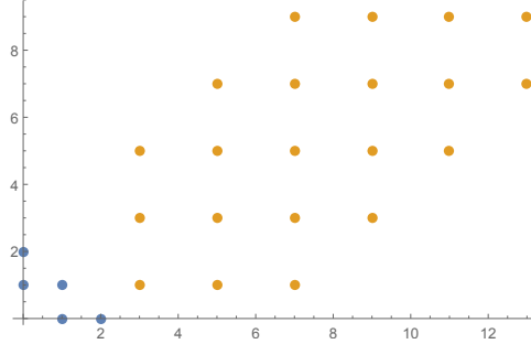
FIGURE 11. The points (i, j) in blue and (m, n) in yellow such that s_1^i s_2^j e^{ms_1/2} e^{ns_2/2} appears in the expression for K_7^{\text{num}} .
