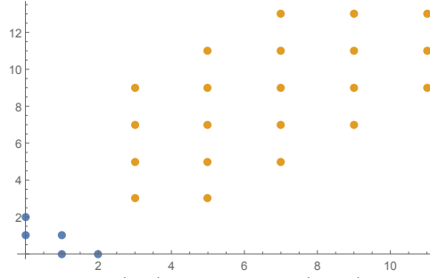
FIGURE 9. The points (i, j) in blue and (m, n) in yellow such that s_1^i s_2^j e^{ms_1/2} e^{ns_2/2} appears in the expression for K_6^{\text{num}} .
