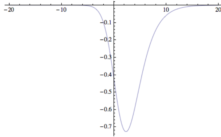
FIGURE 3. Graph of K_1 .
