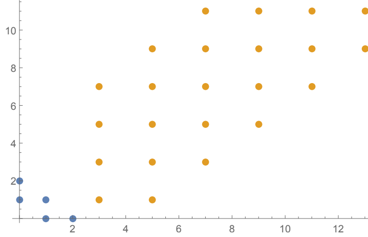
FIGURE 7. The points (i, j) in blue and (m, n) in yellow such that s_1^i s_2^j e^{ms_1/2} e^{ns_2/2} appears in the expressions for K_4^{\text{num}} and K_5^{\text{num}} .
