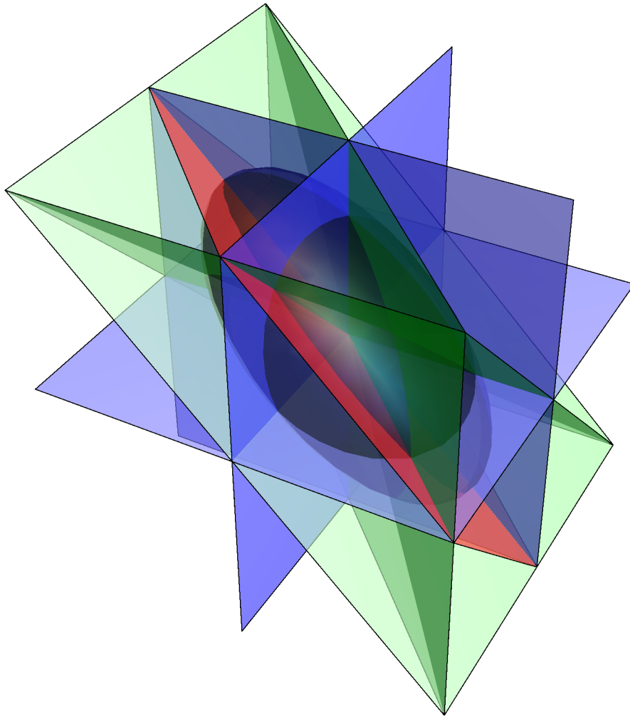
FIGURE 2. The black ellipsoid is the unit ball for the quadratic form Q_3 and the various planes are: in blue the s_j = 0 , in red s_1 + s_2 + s_3 = 0 and in light green the plane s_1 + s_3 = 0 in which the generator of the action of \mathbb{Z}/4\mathbb{Z} is a rotation of angle \pi/2 . The remaining two planes in dark green correspond to the product (s_1 + s_2)(s_2 + s_3) .
