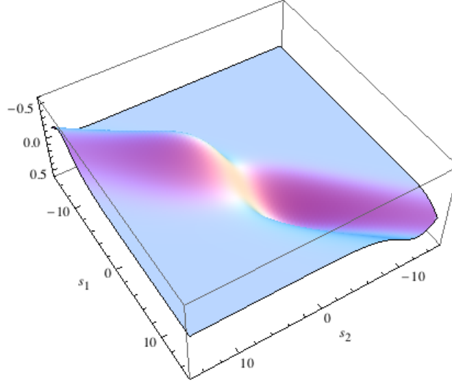
FIGURE 4. Graph of K_3 .
