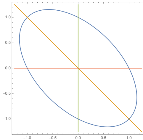
FIGURE 1. The blue ellipse is the unit ball for the quadratic form Q_2 , and the orange, green and yellow lines are respectively the lines s_1 = 0 , s_2 = 0 , and s_1 + s_2 = 0 .
