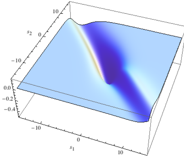
FIGURE 12. Graph of K_7 .
