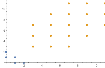
FIGURE 5. The points (i, j) in blue and (m, n) in yellow such that s_1^i s_2^j e^{ms_1/2} e^{ns_2/2} appears in the expression for K_3^{\text{num}} .
