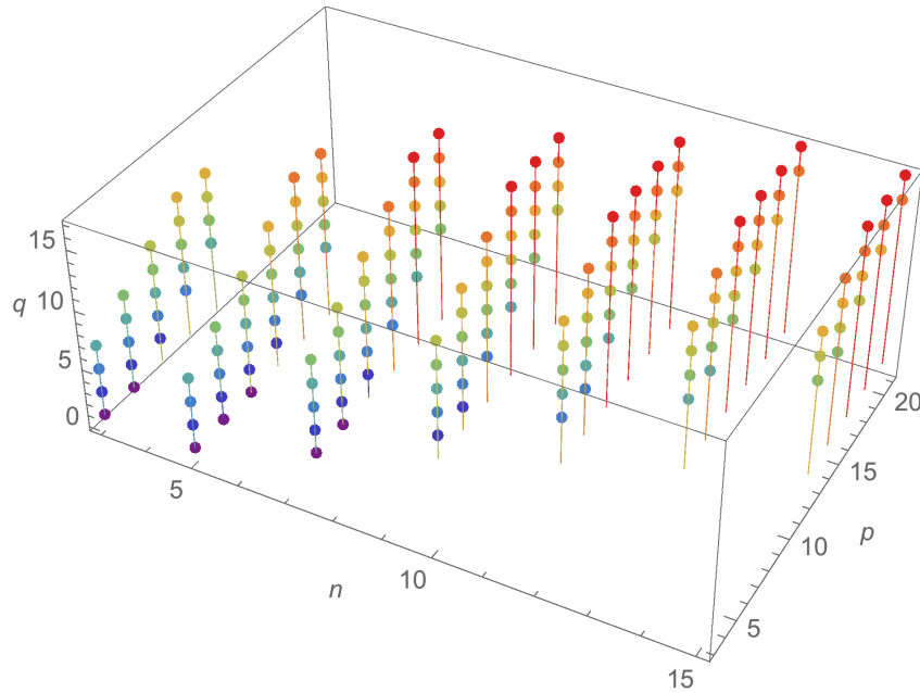
FIGURE 15. The points (n, p, q) such that s_1^i s_2^j s_3^m e^{ns_1/2} e^{ps_2/2} e^{qs_3/2} appears in the expressions for K_8^{\text{num}} and K_{15}^{\text{num}} .
