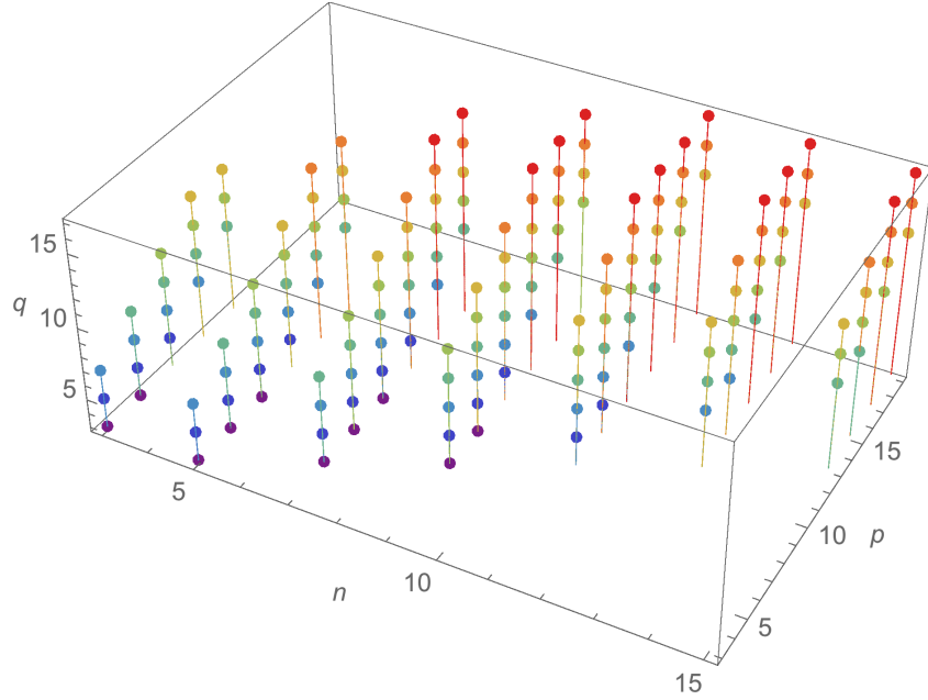
FIGURE 16. The points (n, p, q) such that s_1^i s_2^j s_3^m e^{ns_1/2} e^{ps_2/2} e^{qs_3/2} appears in the expression for K_9^{\text{num}} .
