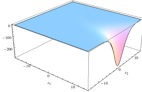
FIGURE 10. Graph of K_6 .
