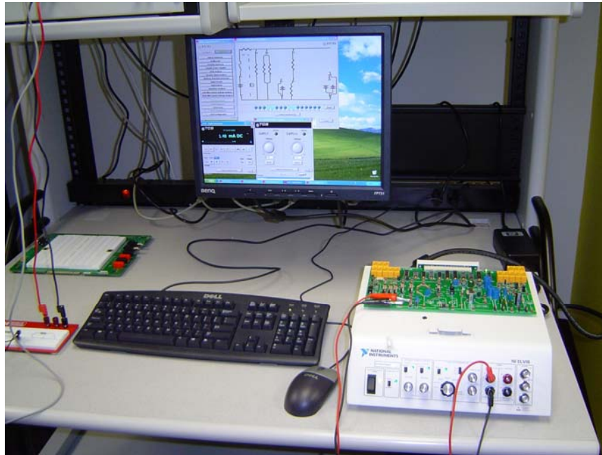
Figure 2. LabVIEW controller for electronics laboratory
