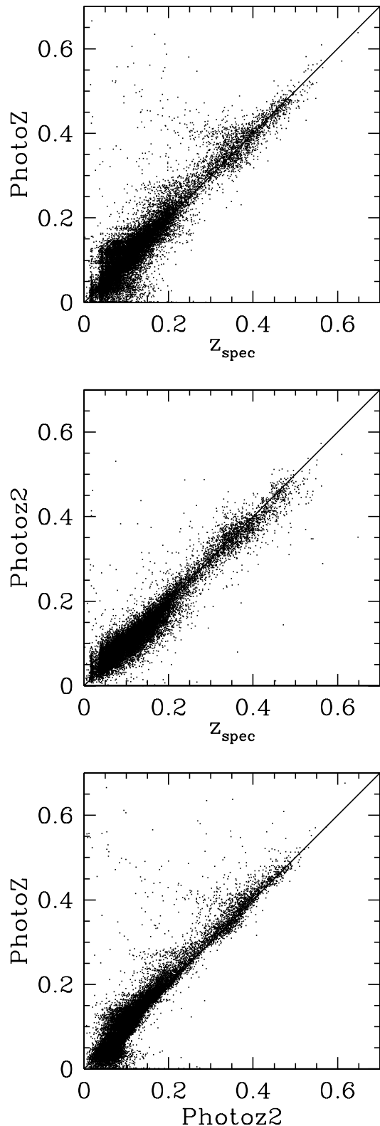
FIG. 6.—Comparison of photometric redshift estimates \text{PhotoZ} and \text{PhotoZ2} to SDSS spectroscopic redshifts and to each other.
