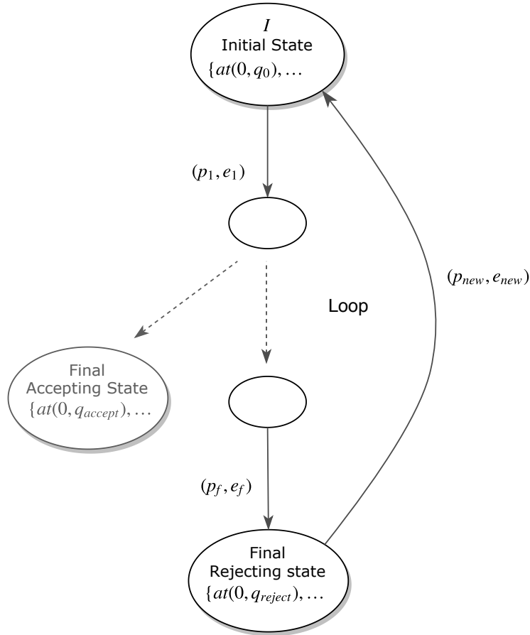
Figure 4: Non-terminating system
