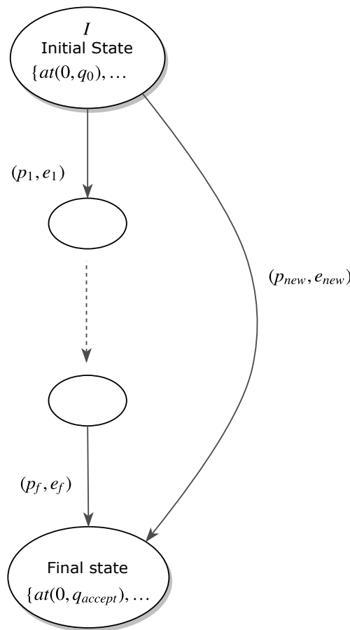
Figure 3: Confluent system
