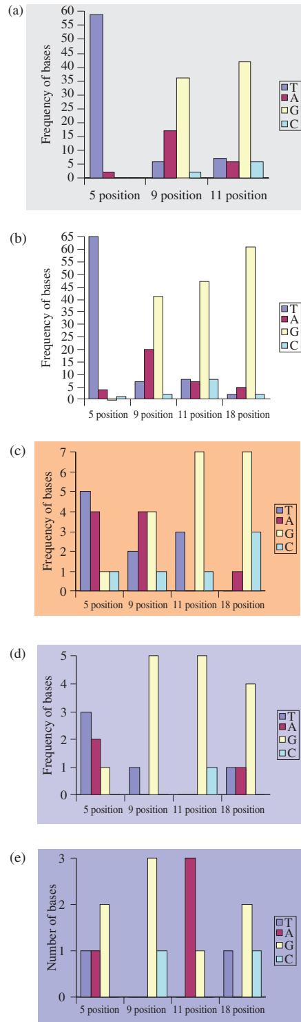
Figure 2. (a) Variations at the 5, 9 and 11 positions, Figure 2 (b) variations at the 5, 9, 11 and 18 positions (c) variants at the 5, 9, 11 and 18 position when A1 and T12 are transposed to T1 and A12, (d) variants at the 5, 9, 11 and 18 positions with G1 and C12 and (e) variants at the 5, 9, 11 and 18 positions with C1 and G12.
