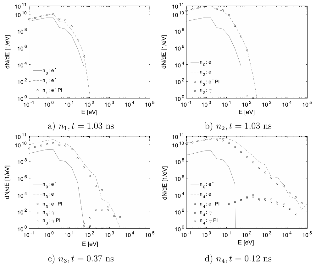
Figure 2. The energy distribution of electrons and bremsstrahlung photons for the time steps shown in Figure 1. The electron energy distribution in uniform air density n_0 (solid), in perturbed air without pre-ionization n_{j=1-4} (dashed), and with pre-ionization (circles). The photon energy distribution in perturbed air without pre-ionization ionization (crosses) and with pre-ionization (squares).
