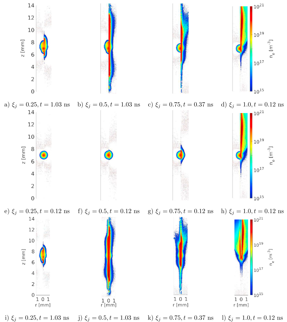
Figure 1. The electron density of streamers for different levels of air density perturbations without pre-ionization (a-h) after the maximum simulated time (a–d) and after 0.12 ns (e–h). The left half of each panel shows the electron density in uniformly distributed air n_0 and the right half in perturbed air n_{1-4} (1). (i–l) Electron density in perturbed air with pre-ionization of n_{e,0} = 10^{12} \text{ m}^{-3} (left) and without pre-ionization (right).
