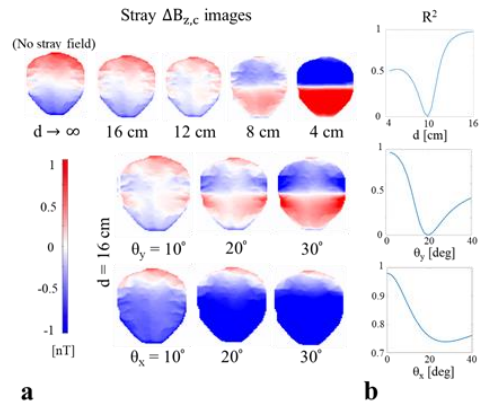
Figure 4. Biot-Savart simulations of the cable-current-induced stray fields. (a) The desired \Delta B_{z,c} image without stray fields (left) is compared with \Delta B_{z,c} images with stray fields for four different simulations in which the wire segment is placed d = [4, 8, 12, 16] cm away from the imaging region (first row). \Delta B_{z,c} images for cable misalignments \theta_y = [10, 20, 30] degrees in y -direction (second row) and \theta_x = [10, 20, 30] degrees in x -direction (third row). Simulations were performed for d = 16 cm. (b) The coefficients of determination between the stray magnetic fields and the desired \Delta B_{z,c} image without stray fields.
