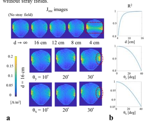
Figure 5. Projected current density images J_{rec} reconstructed from the Biot-Savart simulations in Figure 4.
