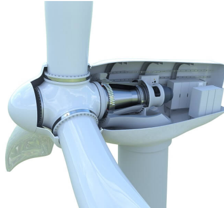
Figure 1.3: Example of drive-train configuration [6]
