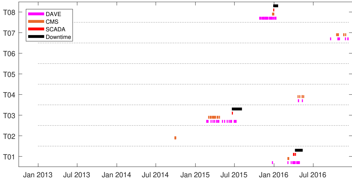
Figure 10: Results for the automated failure detection. Comparing CMS, SCADA and DAVE (FFT1000) alarms.
