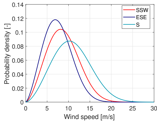
Figure 3.14: Mean wind speed distributions for 3 different directions.
