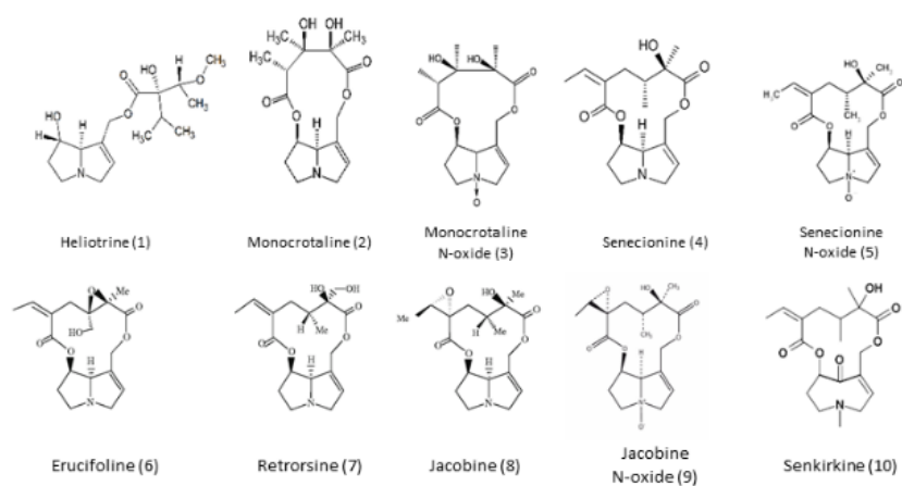
Fig. 1 Chemical structures of selected pyrrolizidine alkaloids.
