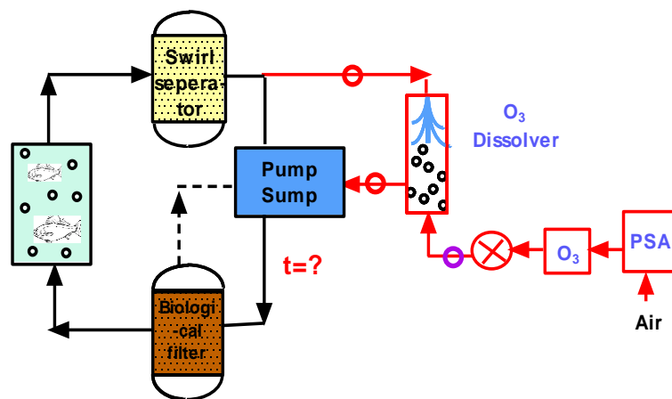
Figure 14: Schematic representation of the pilot-RAS (black lines) with the integrated ozone (red lines).
