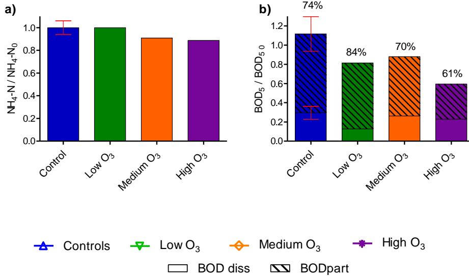
Figure 16: Effect of different ozone dosages, after 8-day-treatment, for the Phase II, on a) TAN, these data could be also found in Paper II, b) BOD 5 (the % and the stripped (upper) part of the bars represents the particulate BOD 5 , while the lower part is dissolved BOD 5 ) in RAS water. The data are normalised and standard deviation applied only in the controls. Modified from Paper IV .
