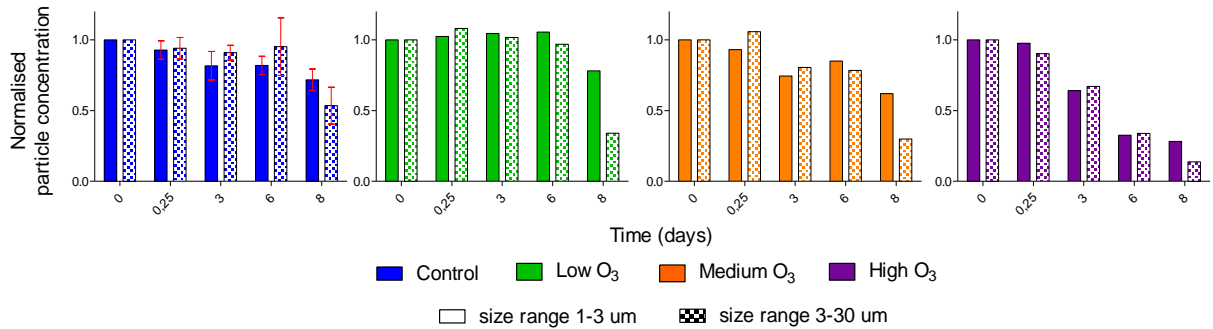
Figure 19: Effect of different ozone dosages on particle size distribution (ranges 1-3 μm and 3-30 μm) and number - normalised data. Modified from Paper IV .
