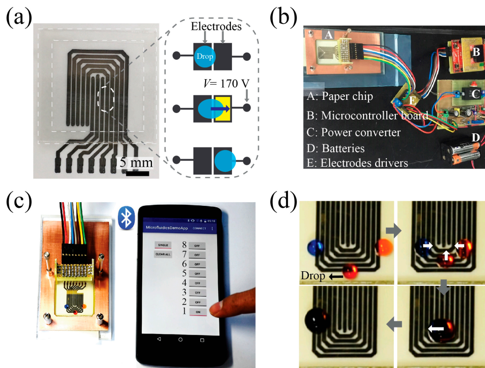
Figure 5. Demonstration of drop actuation on an affordable paper-DMF chip: (a) a printed paper chip and (inset) drop actuation scheme and (b) the chip connected to a power switching device. (c) A smartphone App being run through wireless Bluetooth, and (d) three digital drops initially at rest being simultaneously transported (top) to merge into one drop at the center and then being transported to the left (bottom).
