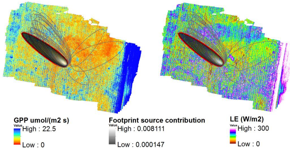
Figure 5-3. An example of the simulated GPP and LE on 25 th May 2016. The circles indicates the variations of the eddy covariance footprint. The shaded area is the footprint location when the UAS flight campaign was conducted. The value in the shaded area indicates the source contribution of the footprint.
