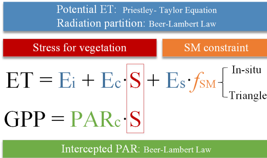
Figure 4-6. Schematic diagram representing the joint PT-JPL ET and LUE GPP model. ‘E i ’ is the evaporation from the intercepted water. ‘E c ’ is the potential transpiration. ‘S’ stands for the vegetation stressors. ‘E s ’ is the potential evaporation from soil. The soil moisture constraint ‘f SM ’ can be obtained from either in-situ observations or the temperature-vegetation triangle approach.
