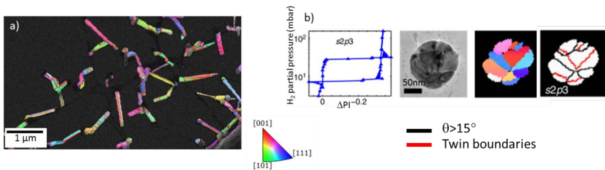
Figure 1: a) TKD orientation map of InP nanowires b) single particle isotherms with TEM and TKD micrographs[4].
