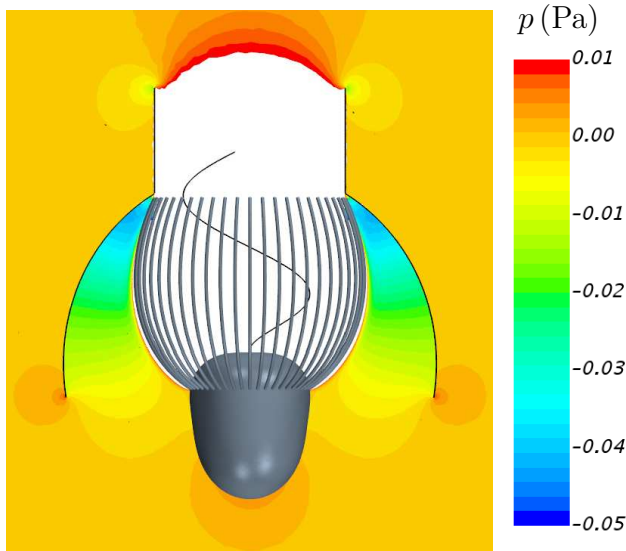
FIG. 6: The time-averaged pressure field in the xz -plane around the freely swimming D. grandis reveals a low pressure region right below the lorica dome which results in a pressure force in the swimming direction. For clarity, the pressure inside the filter and chimney is not shown.
