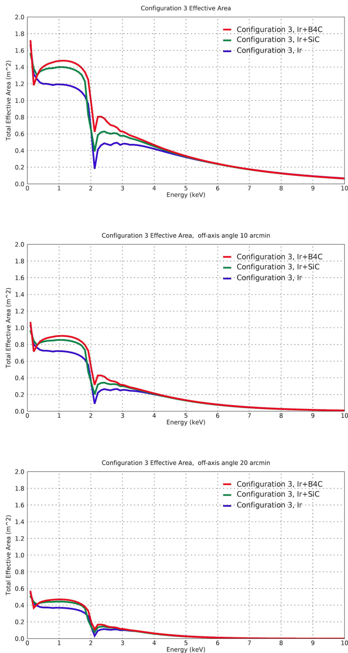
Figure 3. Energy-dependent Effective Area of ATHENA, configuration 3, as computed for three different coatings. The old configuration coating baseline Ir/B 4 C (red curve), the new coating baseline Ir/SiC (green curve), and a plain Ir coating (blue curve) are shown. Top panel: results for an on-axis source. Central panel: results for a 10 arcmin off-axis source. Bottom panel: results for a 20 arcmin off-axis source.
