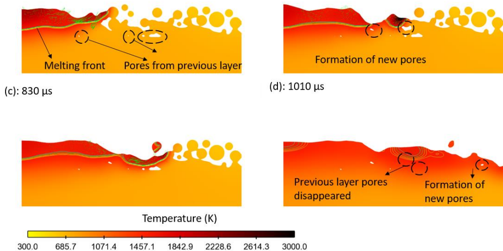
Fig. 9. Fluid region, temperature contour and melt pool dynamics during the scanning of the second layer at y=200\ \mu\text{m} (longitudinal cross-section) at: (a) 730\ \mu\text{s} , (b) 790\ \mu\text{s} , (c) 830\ \mu\text{s} and (d) 1010\ \mu\text{s} .
