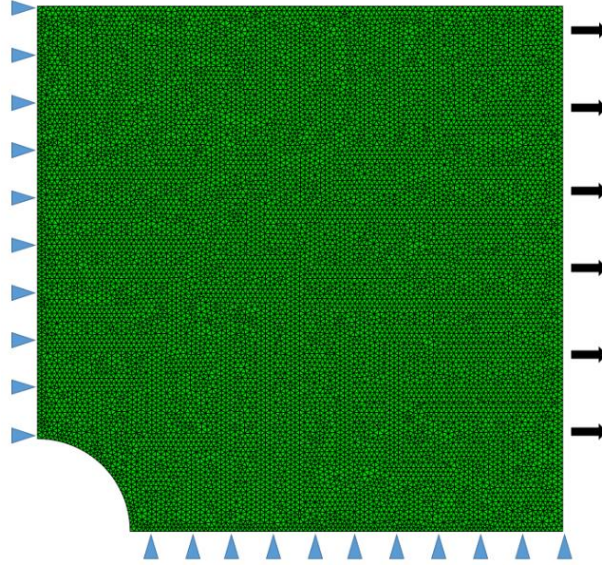
Fig. 4. Mechanical boundary conditions for the unit cell.
