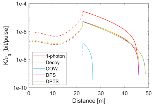
Fig. 3. NLOS secret key rate as a function of the distance for different QKD protocols. Dashed lines are key generations under the condition \theta_i < \theta_c . Full lines under the condition of TIR, i.e. unconditionally secure communications. Parameters used are reported in Table I.
