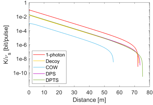
Fig. 2. LOS secret key rate as a function of the distance for different QKD protocols. Parameters used are reported in Table .
