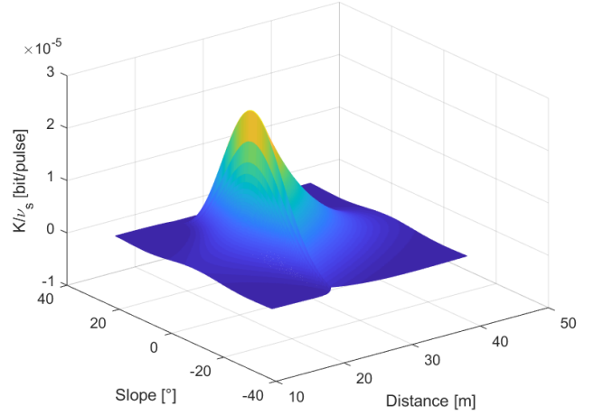
Fig. 4. Secret key rate for NLOS configuration as a function of the upwind/downwind slope. Parameter are reported in Table I.
