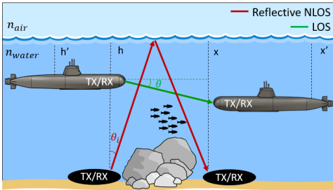
Fig. 1. Underwater link scenarios. Line of sight (LOS) underwater communication between moving vehicles. Non-line-of-sight (NLOS) underwater communications for sensors on the seabed.
