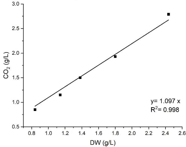
DW vs. accumulated CO 2 from cultivation of T. atrovirens at pH 5.
