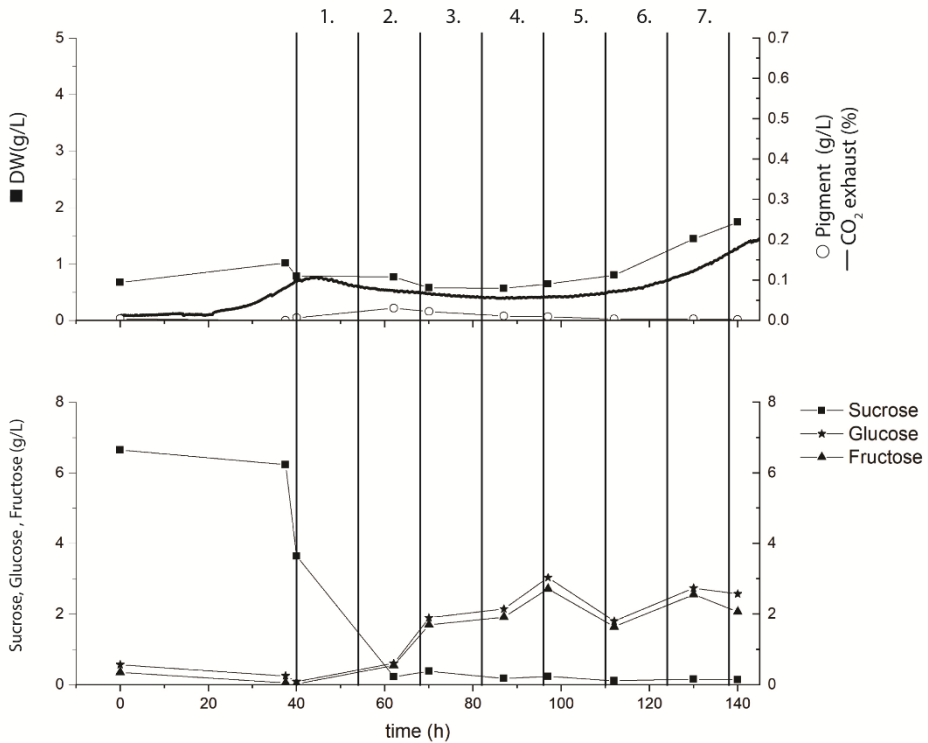
Figure 5.12 Representative chemostat profile for T. atrovirens on \text{KNO}_3 at pH 5 and a dilution rate of D = 0.07 \text{ h}^{-1} . Cultivation conditions were 30 \text{ }^\circ\text{C} with 1 vvm and 800 rpm.
