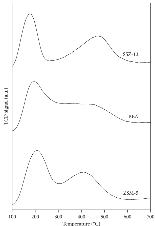
FIGURE 1: NH 3 -TPD profiles of zeolite supports.
