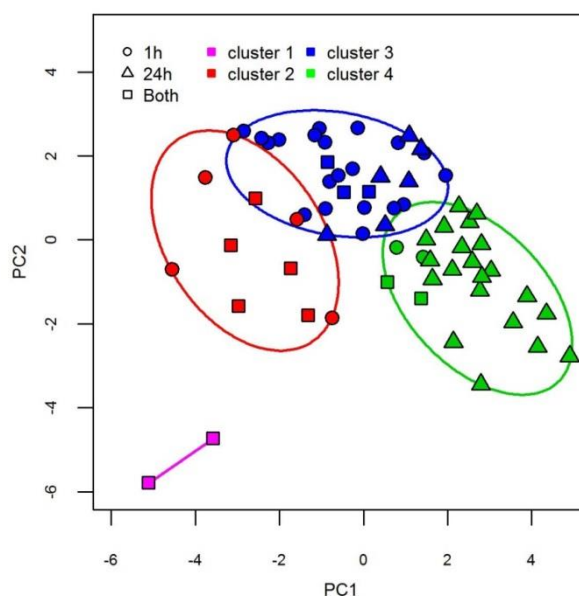
Fig 1: Statistical clustering of extreme events. Cluster 1: Extreme convective, cluster 2: Convective, cluster 3: Convective events within frontal systems, and cluster 4: Frontal system events. Modified from Thomassen et al. (2018).
