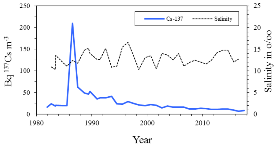
Fig. 4.1. Caesium-137 in seawater collected in Roskilde Fjord 1980 - 2018. (Unit: \text{Bq m}^{-3} )
