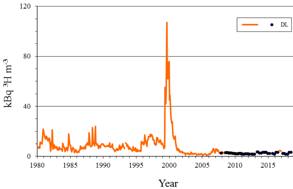
Fig. 4.2. Tritium in seawater collected in Roskilde Fjord 1980 - 2018. (Unit: \text{kBq m}^{-3} ; DL = detection limit)
