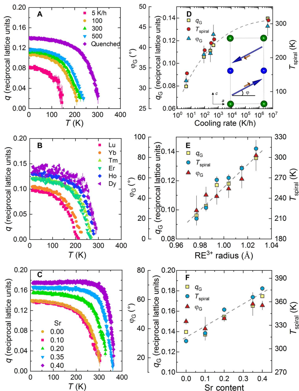
Fig. 3. Evolution of magnetic spiral properties with different tuning parameters. (A to C) Temperature dependence of the magnetic modulation vector q in YBaCuFeO 5 using different tuning parameters: (A) Cooling rate [adapted from (21)]. (B) Replacement of Y 3+ by a rare-earth cation (RE 3+ ). (C) Replacement of Ba 2+ by Sr 2+ . (D to F) Evolution of T_{\text{spiral}} , the ground-state values (10 K) of the magnetic modulation vector ( q_G ), and the inclination of the spiral rotation plane ( \phi_G ) using different tuning parameters: (D) Cooling rate [adapted from (21)]. (E) Replacement of Y 3+ by a rare-earth cation (RE 3+ ). (F) Replacement of Ba 2+ by Sr 2+ . The inset in (D) shows the definition of the inclination angle \phi_G . The dashed lines are guides to the eye and indicate the positive correlation among T_{\text{spiral}} , q_G , and \phi_G . The values for REBaCuFeO 5 and YBa 1-x Sr x CuFeO 5 families were extracted from Rietveld fits of the DMC data recorded at 10 K (fig. S5). The error bars of q_G and \phi_G , listed in tables S2 and S3, are the SDs obtained from the fits of the magnetic structure using the FullProf Suite Rietveld package (50).
