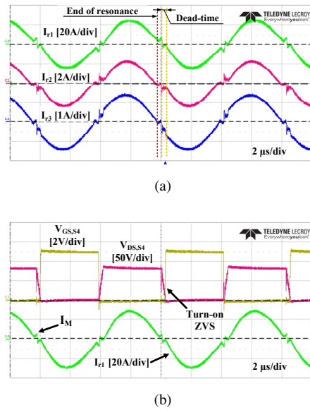
Fig. 12. Experimental results obtained in steady-state at 1.2 kW in dual-output mode with Port-1 ( V_1 = 80 V) operating as input. (a) Tank circuit currents, (b) Tank current at input side, drain-source voltage and gate-source voltage of MOSFET S_4 .
