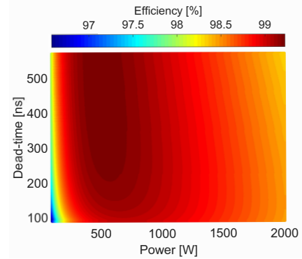
Fig. 9. Analysis of the TP-SRC efficiency in terms of t_d and power level. Efficiency is calculated for dual-output mode with LV side as input at f_{sw} = 150 kHz with L_{r,HV} = 1.5 \mu\text{H} .
