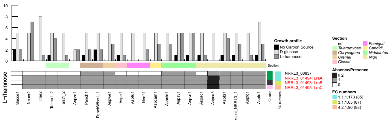
Fig. 11. L-rhamnose heatmap abundance of A. niger orthologous proteins in the L-rhamnose catabolic pathways. The legends are the same as that of Fig. 3.
