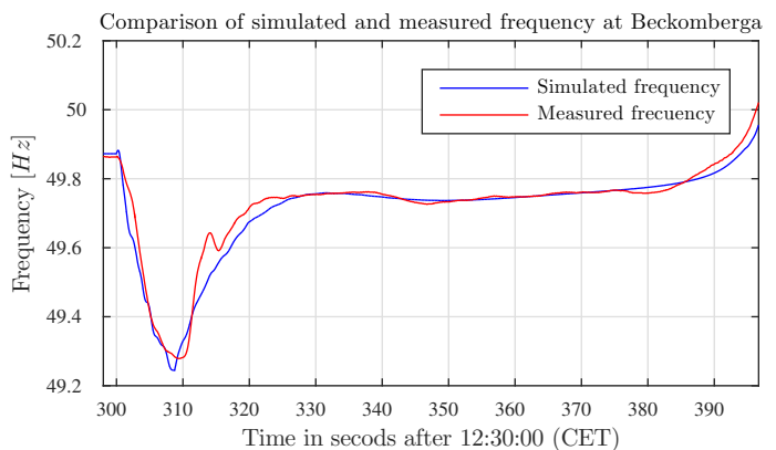
Fig. 5. Simulated results of system frequency held against measured values of the frequency from the blackout.
