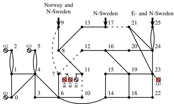
Fig. 4. The system condition after the double busbar fault in Horred (bus 7). As a consequence, practically no local production was available in the southern part of Sweden (buses 6,7,10,14-16,18-24). The power was either supplied from Denmark (through bus 6) or from North (through bus 25).
