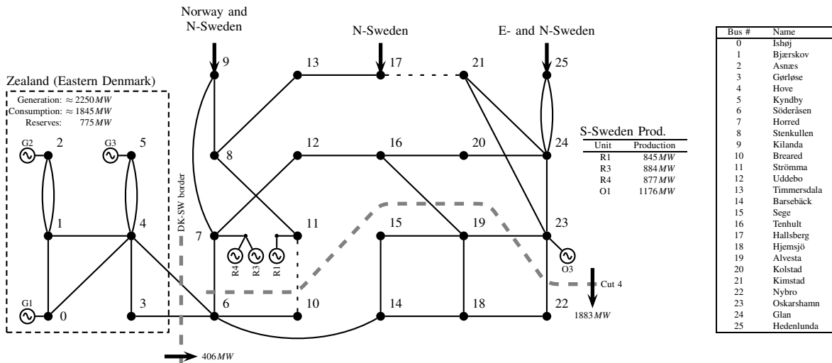
Fig. 2. The pre-fault conditions in the the 400kV grid in E-Denmark and S-Sweden. The generators in Zeeland represent an aggregation of several generators in corresponding area, while the generators in Swedish part represent the individual generating units that where operating prior to the blackout.
