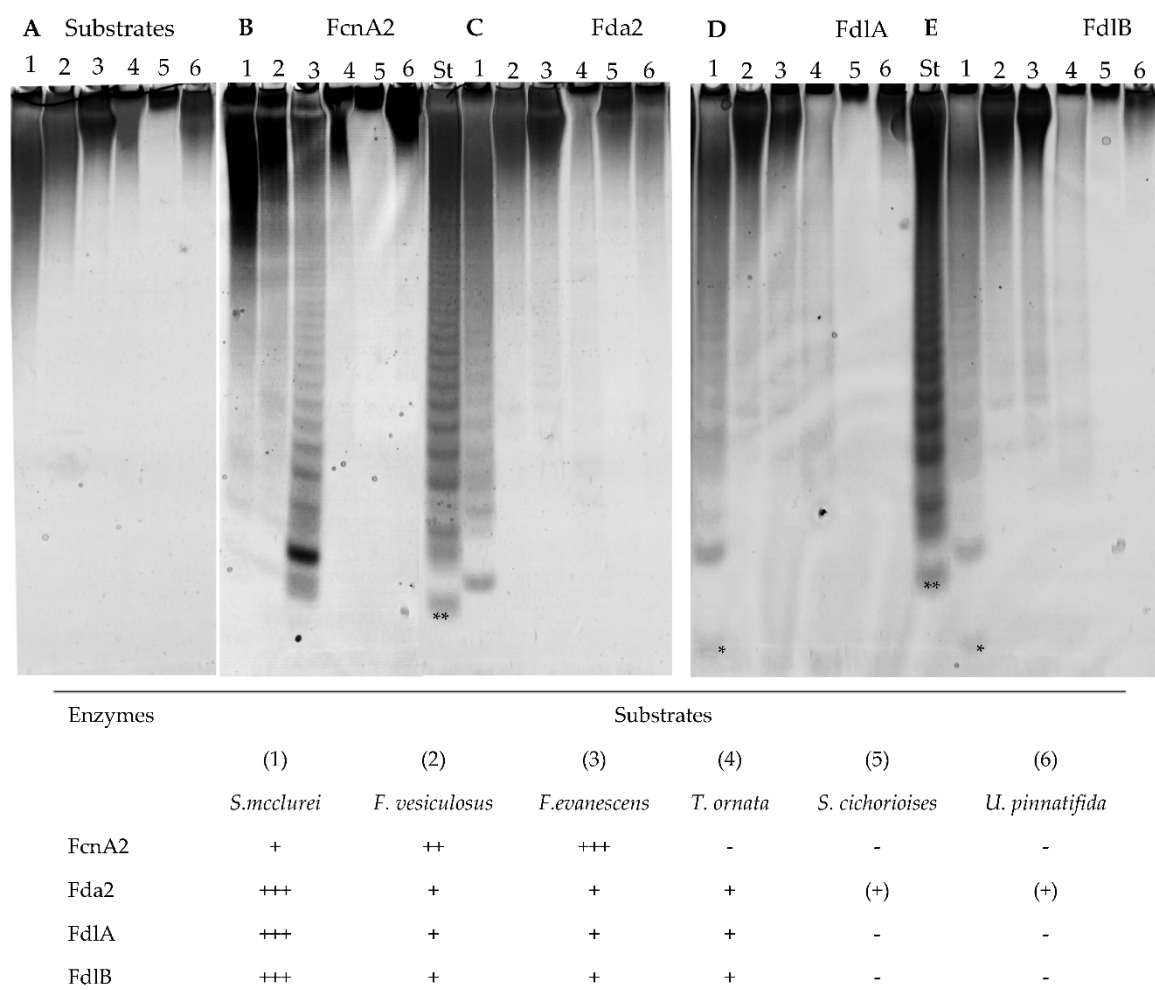
Figure 3. C-PAGE analysis of fucoidan degradation using purified enzymes: (A) substrate control with no enzyme; and (B–E) enzymatic products from reaction of FcnA2, Fda2, FdIA, and FdIB on different fucoidans, respectively (expression of recombinant Fda1 resulted in insoluble enzymes, which is why there are no data for Fda1): (1) Sargassum mcclurei ; (2) Fucus vesiculosus ; (3) Fucus evanescens ; (4) Turbinaria ornata ; (5) Saccharina cichoriooides ; and (6) Undaria pinnatifida . The extent of degradation is indicated with: (+++) highest, (++) medium, (+) lowest and (+) is positive activity resulting in a high molecular smear, while (–) is no activity. The standard (St) is the product profile of FFA2 treatment of fucoidan from F. evanescens . The lowest band (**) of the St is a tetra-saccharide of (1→4)- and (1→3)-linked \alpha -L-fucosyls sulphated at every C2 with an approximate mass of 972 Da [27]. (*) indicates an enzymatic fucoidan degradation product of either lower mass or higher charge than the lowest St band (**). The reaction time was 24 h.
