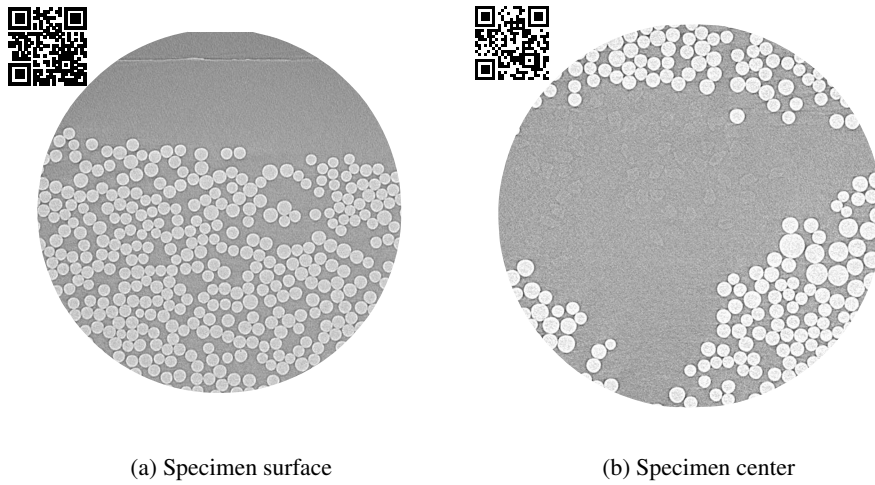
Figure 8: Small field of view scans of a reference specimen.
