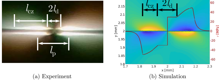
Figure 1: A fiber break as observed during an experiment and through numerical simulation, showing the quantities of interest for property estimation.
