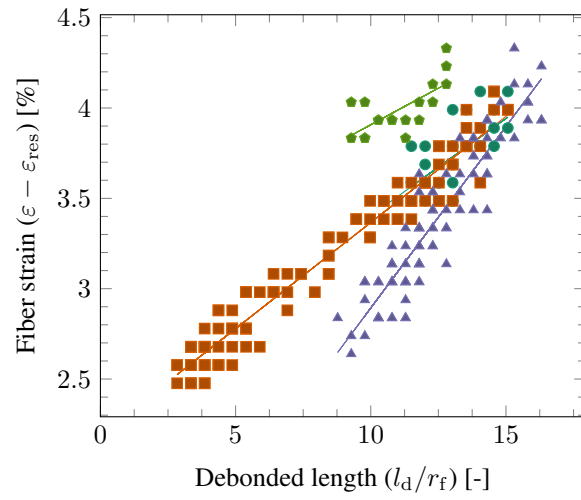
Figure 2: SFFT results for dry specimens.
