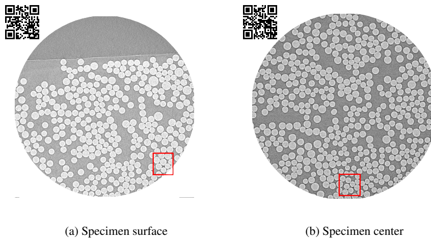
Figure 11: Small field of view scans of a specimen aged at 50 °C, with small debonding cracks marked in red.
