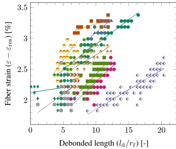
Figure 3: SFFT results for saturated specimens.
