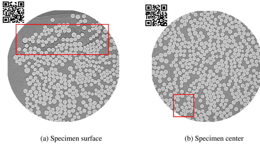
Figure 10: Small field of view scans of a specimen aged at 65 °C, with cracks marked in red.
