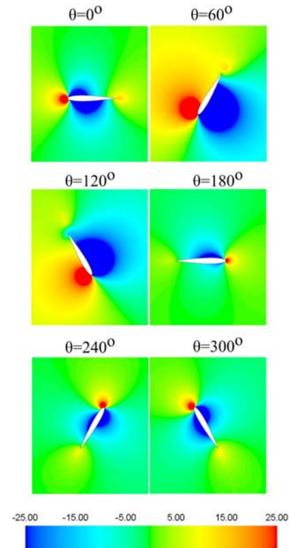
Fig. 12. Contours of instantaneous static pressure at six azimuthal positions.
