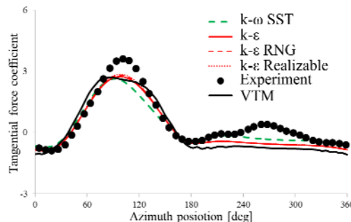
Fig. 7. Tangential loads vs. azimuth position. The comparison between CFD, the experimental data (Strickland et al. (1981)) and the Brown's Vorticity Transport Model (Scheurich et al. (2011)).
