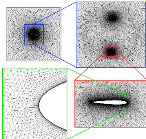
Fig. 5. Mesh distribution for CFD simulation.
