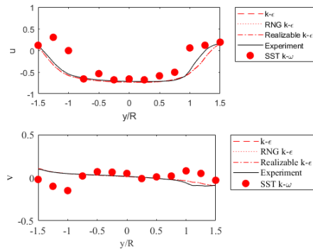
Fig. 15. Velocity profiles at the azimuth position of 30° for four turbulence models.
