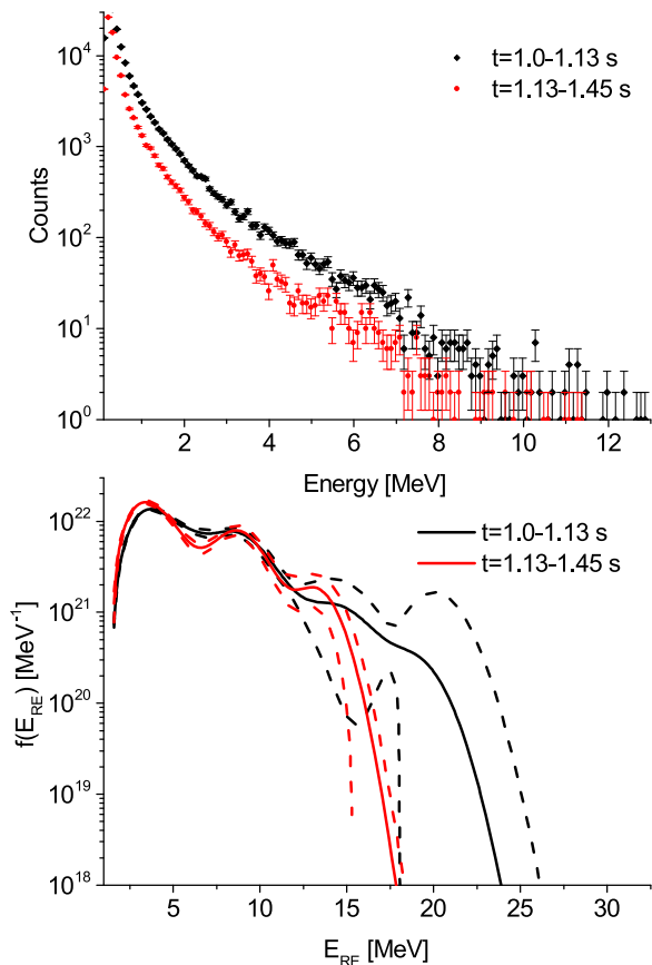
FIG. 4. (Top) Hard x-ray bremsstrahlung spectrum measured for discharge #34084 with MGI in the time windows t = 1.0\text{-}1.13 s and t = 1.13\text{-}1.45 s. (Bottom) Runaway electron distribution functions obtained by the deconvolution of the data shown in the top figure. The dashed lines indicate the statistical uncertainty level.
