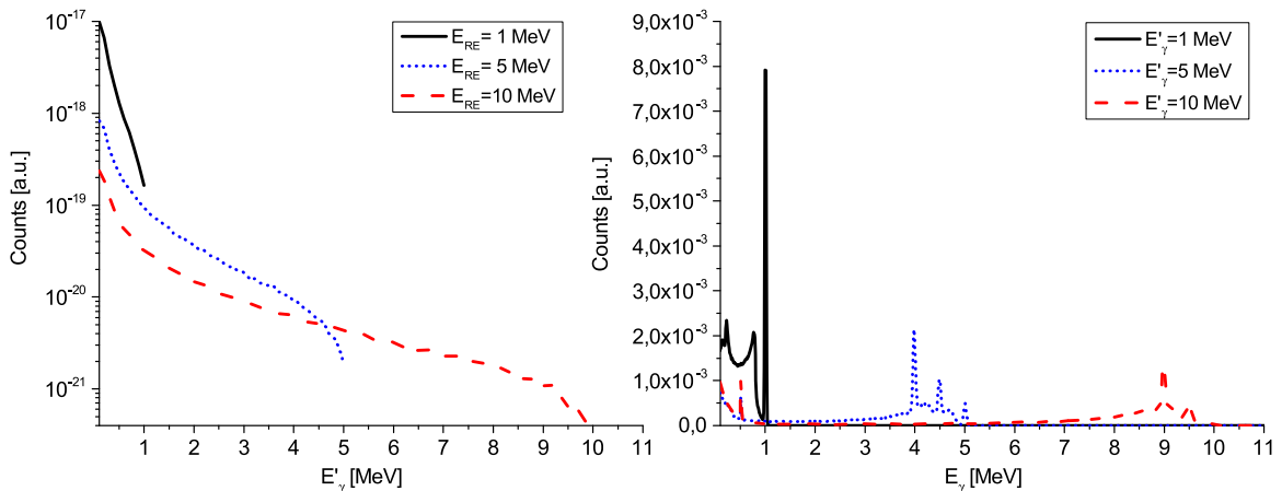
FIG. 2. (Left) HXR bremsstrahlung spectrum g(E'_\gamma, E_{RE}) generated by monoenergetic runaway electrons at energies E_{RE} = 1, 5, and 10 MeV. (Right) Response function of the \text{LaBr}_3 detector used at ASDEX Upgrade: d(E_\gamma, E'_\gamma) to monoenergetic gamma-rays at energies E'_\gamma = 1, 5, and 10 MeV.
