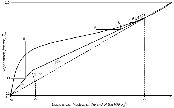
Fig. 2. McCabe-Thiele constructions for the cyclic distillation (stage 12 is the reboiler).
