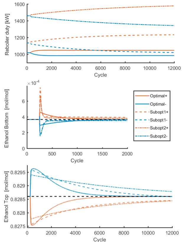
Fig. 4. The closed loop process response of the optimal process design and suboptimal process designs to \pm 10\% change in feed flow rate.
