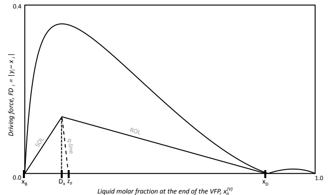
Fig. 1. Driving force diagram for the separation of ethanol-water mixture.
