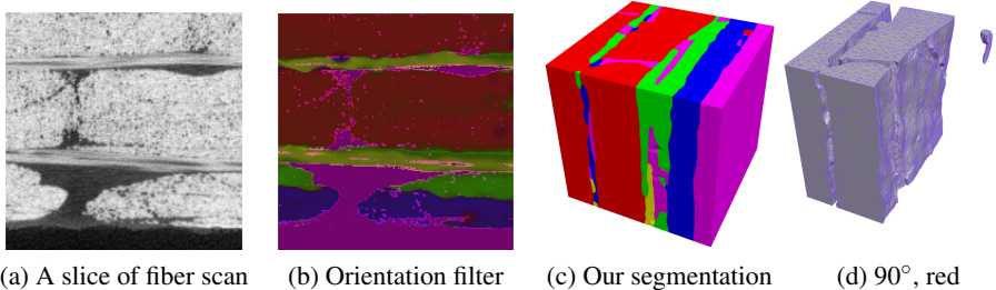
Figure 8: Fiber bundle segmentation, utilizing fiber orientation filter. Color codes: red is 90^\circ bundle, green is 45^\circ , blue is 0^\circ , yellow is -45^\circ , and pink is the resin. We demonstrate the mesh of phase 1 ( 90^\circ orientation) in (d)
