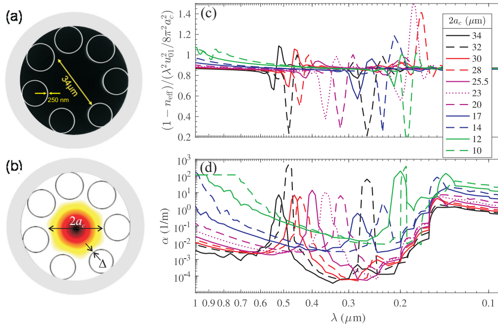
Fig. 1. (a) SEM image of a fabricated HC-AR silica fiber with 7 AR cladding tubes, 250 nm tube-wall thickness and 34 \mu\text{m} core diameter. (b) The FEM design used in this paper is based on the fiber (a), and the FEM structure is shown overlapped with the fundamental mode at 800 nm. (c) and (d) FEM data of calculated effective index for an evacuated fiber and loss vs. wavelength. The effective index is scaled to the vacuum MS dispersion, see text for details. The original fiber ( 2a_c = 34 \mu\text{m} and \Delta = 250 \text{ nm} ) was used as a starting point, and the shown cores sizes are then considered linearly tapered so \Delta is scaled accordingly down.
