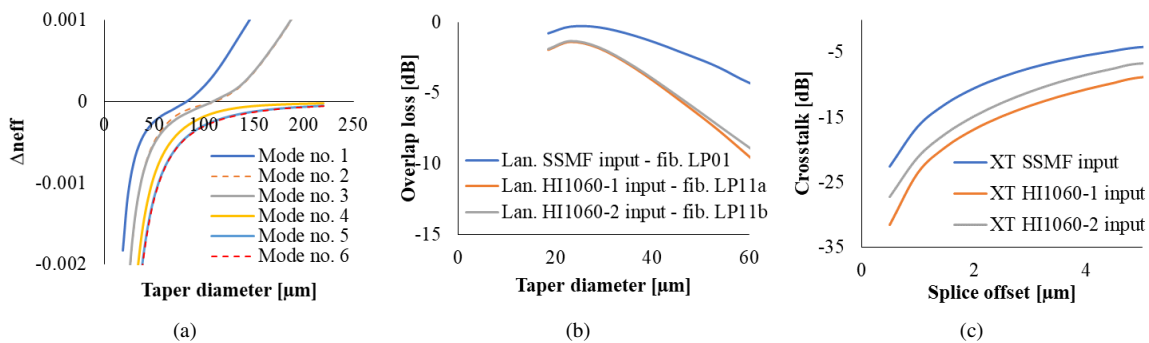
Fig. 1. Result of simulations. a) effective index difference versus taper diameter. b) Coupling loss between end of taper and two mode fiber due to mismatch in mode distributions. c) Effect of offset in the coupling of taper end and two mode fiber on mode crosstalk.
