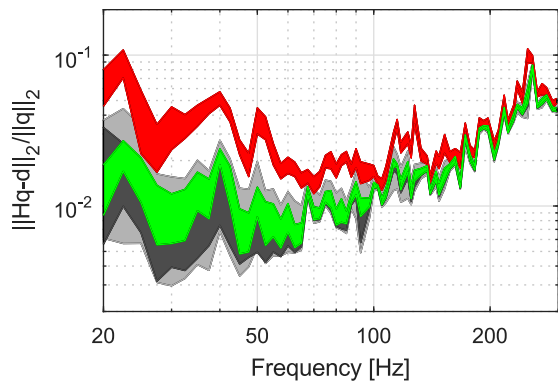
Fig. 3. \ell_2 -norm of the residual error, normalized by the \ell_2 -norm of the loudspeaker weights, calculated at each frequency.
