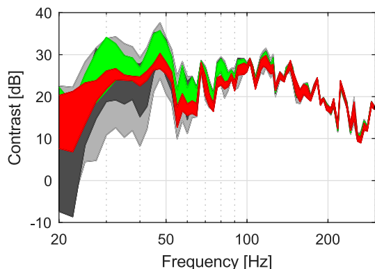
Fig. 4. Ratio of average squared pressure in the bright zone relative to the average squared pressure in the dark zone, displayed in dB.
