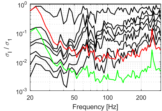
Fig. 2. Black curves: singular values of \hat{\mathbf{H}}[\omega] . Red curve: Maximal singular value of \mathbf{R}_{95\%}[\omega] with K = 1 . Green curve: Maximal singular value of \mathbf{R}_{95\%}[\omega] with K = 29 . All the curves have been normalized by the maximal singular value of \hat{\mathbf{H}}[\omega] at each frequency.
