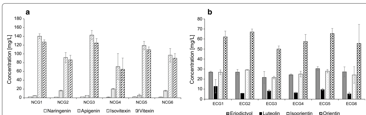
Fig. 3 Indirect C -glycosylation. a NCG strains production of naringenin (white), apigenin (light grey), isovitexin (grey hatching) and vitexin (black hatching). b ECG strains production of eriodictyol (dark grey), luteolin (black), isoorientin (grey checker) and orientin (black checker). Represented are averages and standard deviations of four independent cultures
