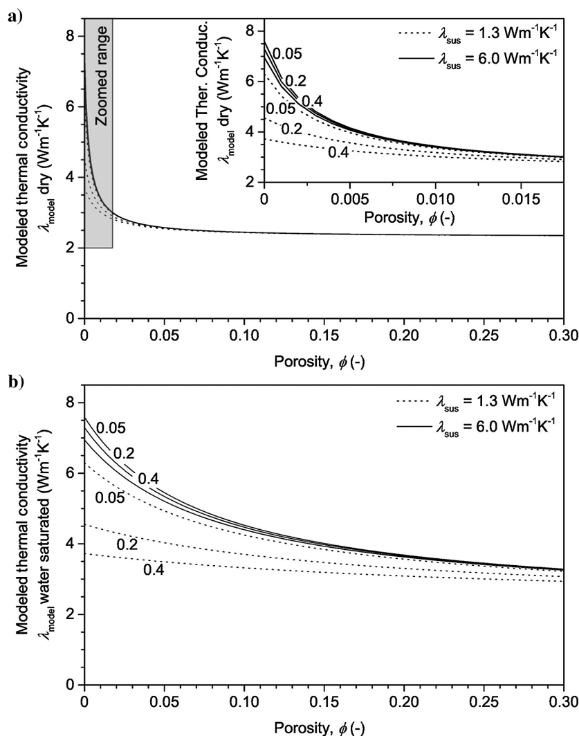
Figure 3. Model predictions of thermal conductivity from equation 7 as a function of porosity using \lambda_{\text{lbs}} = 7.7 \text{ Wm}^{-1} \text{ K}^{-1} for quartz (Clauser and Huenges, 1995) and fixed values of \alpha = 0.7 and c_M after equation 4. Labels on lines indicate V_{\text{sus}} = 0.05, 0.2, \text{ and } 0.4 , respectively. (a) In the dry state, assuming air as saturating fluid and \lambda_f = 0.024 \text{ Wm}^{-1} \text{ K}^{-1} (Beck, 1976), (b) in the water-saturated state, assuming \lambda_f = 0.62 \text{ Wm}^{-1} \text{ K}^{-1} equal to that of pure water (Beck, 1976).
