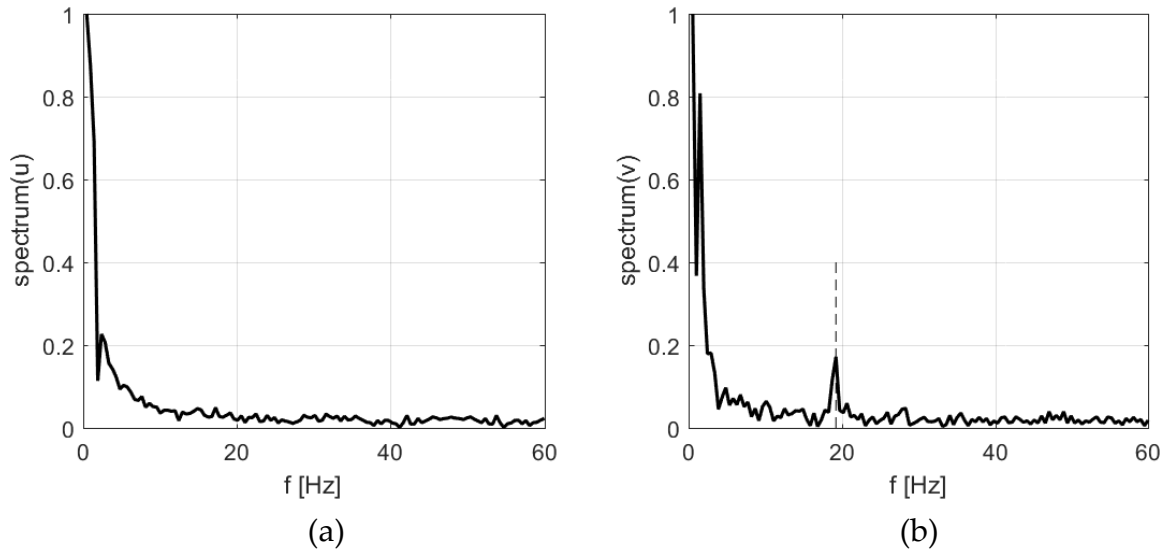
Fig. 8 Spectrum analysis, (a) horizontal velocity u(t) , (b) vertical velocity v(t) .
