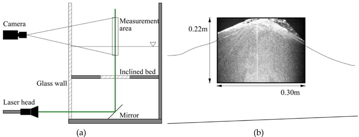
Fig. 2 (a) Cross-sectional view of the wave flume at the PIV / PTV measurement area. The horizontal laser sheet reflects on a 45°-tilted mirror at the bottom of the wave flume and propagates vertically through a window in the inclined, smooth laboratory bed. (b) Field of view of the PIV / PTV measurement area.
