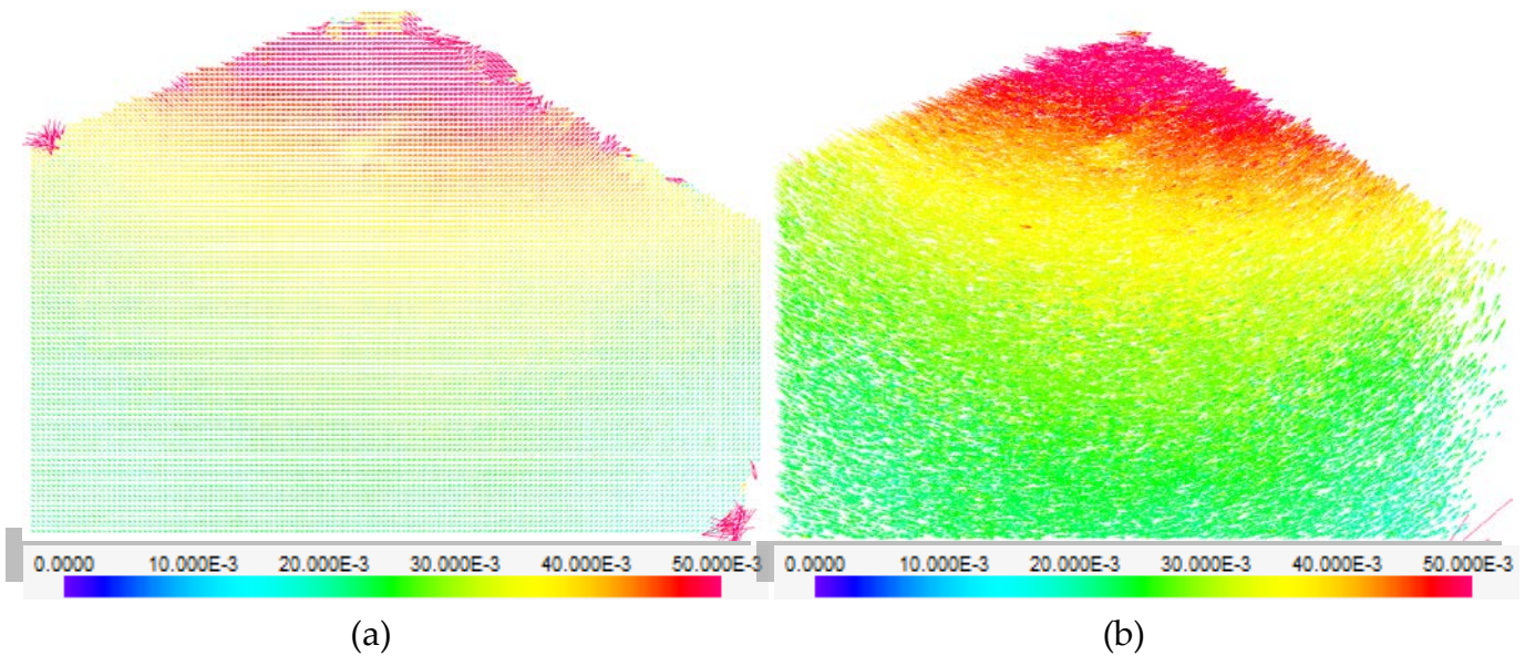
Fig. 5 (a) Preliminary PIV analysis used as input for subsequent PTV analysis. Color bar is arbitrary scale (b) PTV results. Color bar is arbitrary scale. Both at t=0.646s .
