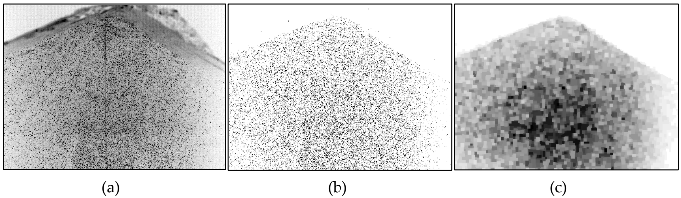
Fig. 4 (a) Inverted raw particle image after background subtraction. (b) After application of Difference of Gaussian filter (c) Pre-processed image used for histogram-threshold based dynamic masking. All at t=0.646s .
