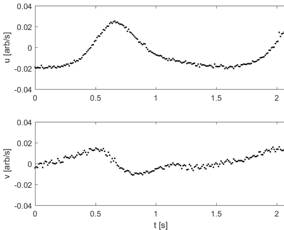
Fig. 7 Velocity time series in the horizontal, u(t) , and in the vertical, v(t) , obtained at the black circle in Fig. 6.
