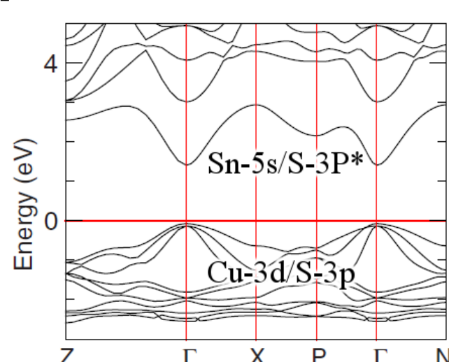
Figure 5: Band diagram of CZTS (kesterite) [9].
