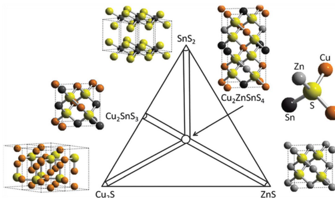
Figure 1: The pseudoternary phase diagram with the kesterite phase and other secondary phases along with their crystal structures [8].
