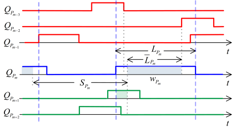
Fig. 5. Guaranteed time slot in an open window.
