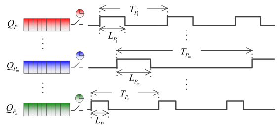
Fig. 4. Open-close cycle and open windows of each queue gate.
