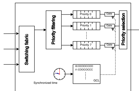
Fig. 1. Simplified view of a 802.1Qbv-capable switch.
