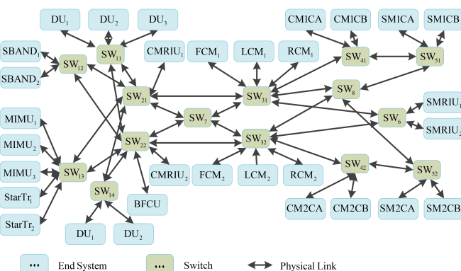
Fig. 13. Network topology of the Orion CEV. [9]
