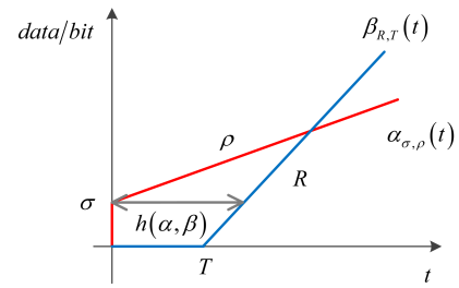
Fig. 3. A simple analysis example by using network calculus.
