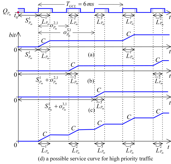
Fig. 7. Worst-case service scenario for high priority traffic based on a benchmark.
