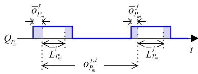
Fig. 10. Relations of relative offsets \bar{o}_{P_m}^i and o_{P_m}^{j,i} .
