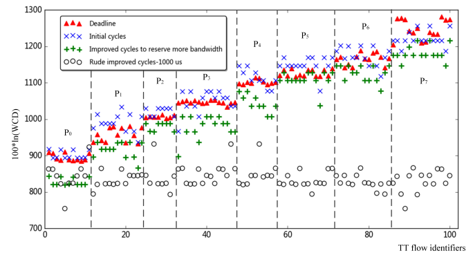
Fig. 14. Compared WCDs under different cycle of GCL of priority queues.
