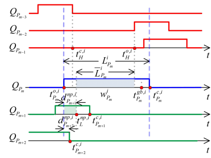
Fig. 8. Guaranteed service time slot \bar{L}_{P_m}^j in an open window w_{P_m}^i .
