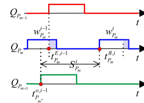
Fig. 11. The maximum waiting time at the beginning busy period.
