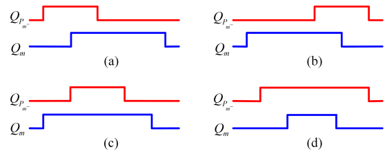
Fig. 9. Overlapped cases of open windows between P_{m-} and P_m .
