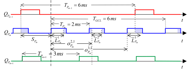
Fig. 6. Guaranteed time slots for P_m .
