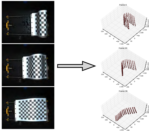
Figure 2.6: Illustration of NRSfM. The general idea is to take a set of 2D observations (typically from images) and produce an estimate of the scene and view geometry. The reconstructions on the right have been created using the algorithm described in [KDL17a]
