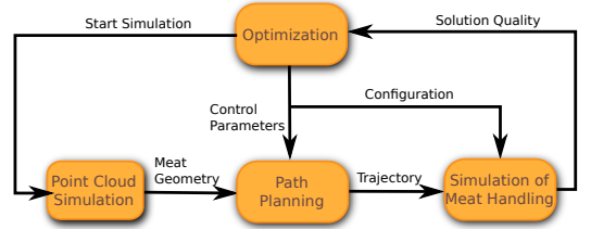
Fig. 3: Diagram of the simulation-based parameter optimization. This process describes how the control parameters and configuration are determined in the parameter tuning block of Fig. 2.
