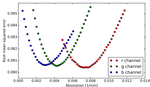
Fig. 12. Analysis by synthesis to estimate absorption of the glass bowl. We run renderings in low resolution and change the absorption in each color channel one at a time. In the case of the bowl, the blue channel is the most sensitive one.
