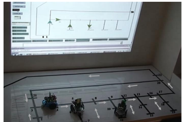
Figure 8. Plant prototype (bottom) and HMI (top)
