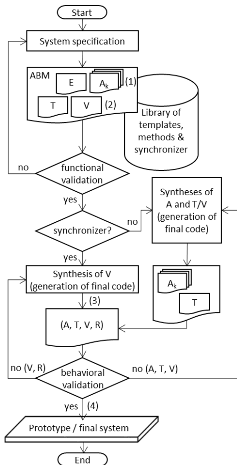
Figure 7. Transportation system controllers' development methodology with and without synchronizers
