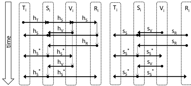
Figure 5. Synchronizer's ( S_i ) event interface protocol for hard (left) and soft (right) real time events
