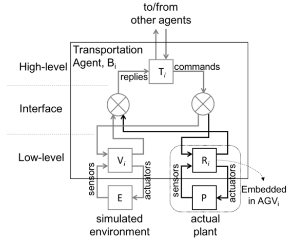
Figure 3. Architecture of transportation agents
