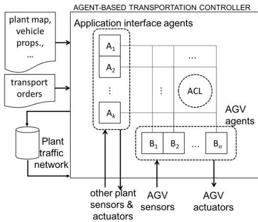
Figure 1. Multi-agent model of a controller for transportation systems
