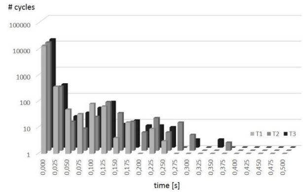
Figure 9. Control cycle execution time logarithmic histogram of three robots, T_1 , T_2 and T_3
