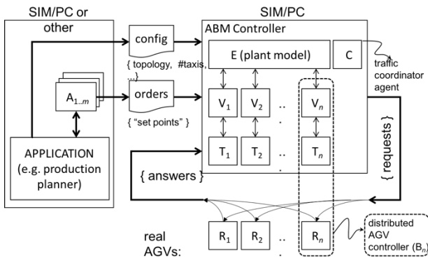
Figure 4. ABM control loop for multi-AGV transport systems
