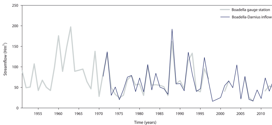
Figure 7. Observed annual streamflow at the Boadella gauge station (grey) and at the Boadella–Darnius dam inflow (blue).
