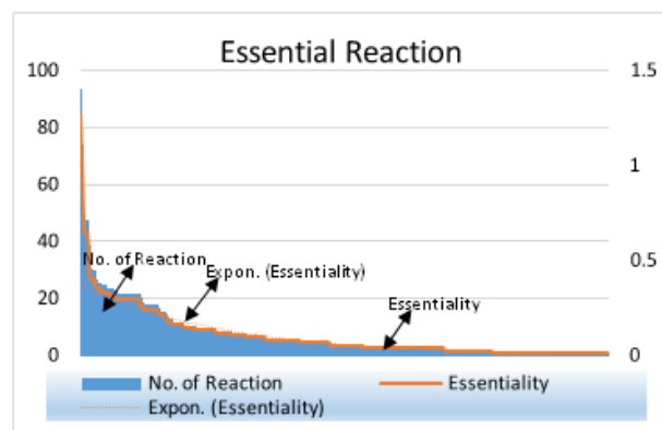
Fig. 1. Graph to show No. of reactions considered and essentiality of reactions.
