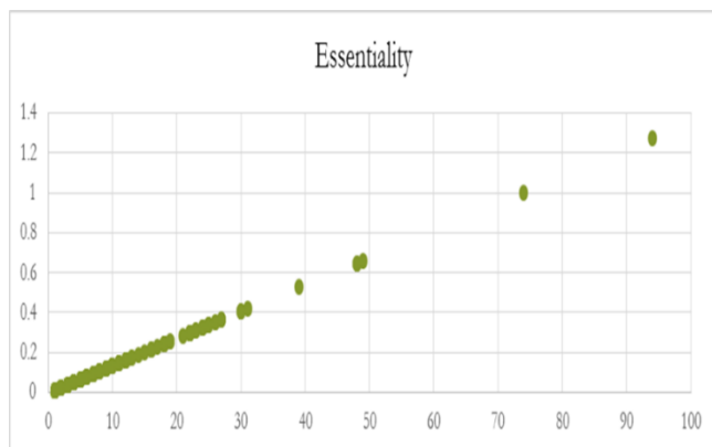
Fig. 2. Graph to represent essentiality of reactions
