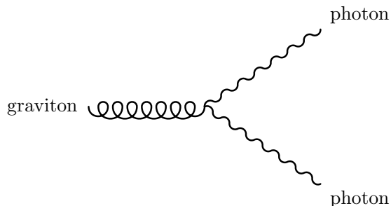
FIG. 3 Allowed tree level graviton decay diagram if the graviton is massive (and one can go in its rest frame).
