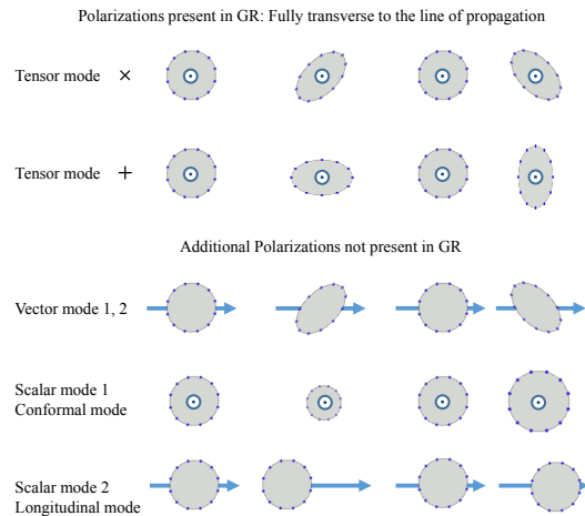
FIG. 1 The six modes for a massive spin-2 field. The two tensor modes and the scalar conformal mode are propagating out of the page; the two vector modes and the longitudinal scalar mode are propagating to the right (taken from (de Rham, 2014)).
