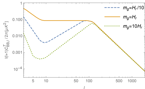
FIG. 2 A schematic sketch of B-mode power spectra for a range of graviton masses (See Fig. 3 of (Dubovsky et al. , 2010) for more details). We use H_r as the Hubble parameter at recombination. A characteristic plateau appears at \ell < 100 when the graviton mass is of the order of the Hubble parameter at recombination. When m_g is much bigger or smaller than H_r , the low \ell power spectrum is, on the other hand, suppressed.
