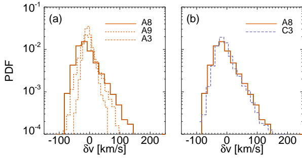
Figure 4. Probability distribution functions of the radial speed with respect to a 30 minute running mean during (a) three flat-tops of the same stream at different radial distances, R \sim 0.3, 0.57, 0.98 AU, and (b) two flat-tops of different streams at \sim 0.3 AU.
