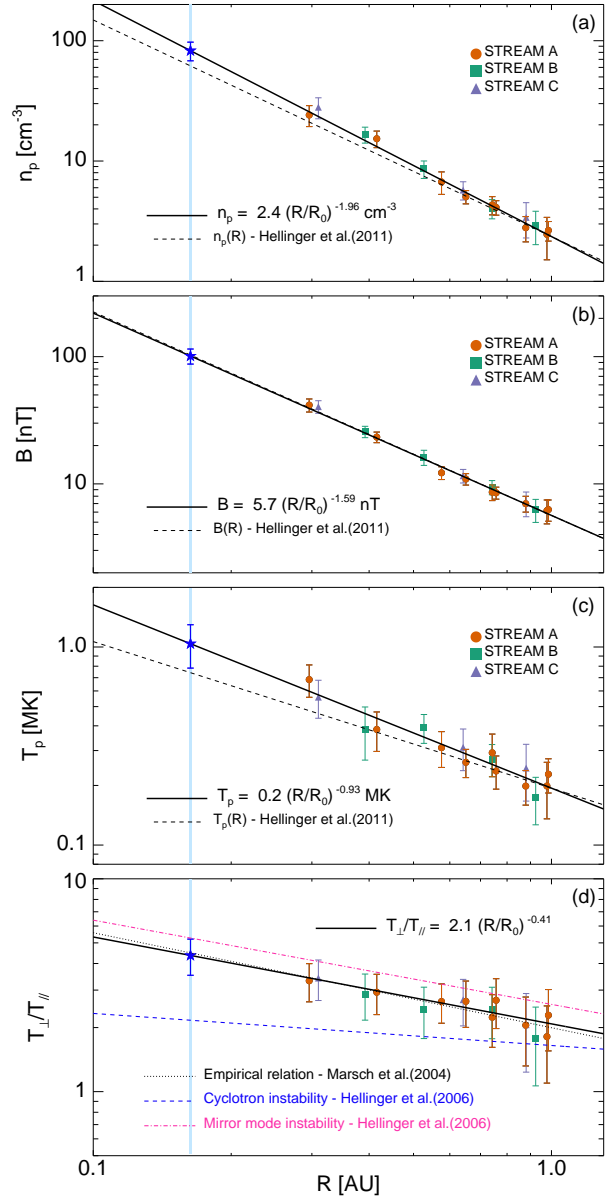
Figure 5. Solar-wind radial evolution: (a) proton density; (b) magnetic field magnitude; (c) proton temperature; and (d) temperature anisotropy. Each point and relative error bar refer to the mean and \pm the standard deviation in each flat-top. Different colours and symbols indicate different streams. Black-solid lines show the fits for the stream A (orange circles). Blue stars refer to extrapolated fast-stream values at \sim 35R_S (blue-filled band).
