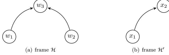
Figure 4: frames \mathcal{H} and \mathcal{H}' in Example 72. D components are omitted for clarity.
