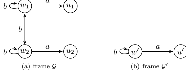
Figure 2: Frames \mathcal{G} and \mathcal{G}' in Example 10.
