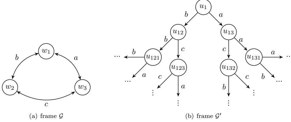
Figure 3: frames \mathcal{G} and \mathcal{G}' in Example 65. D components are omitted for clarity.
