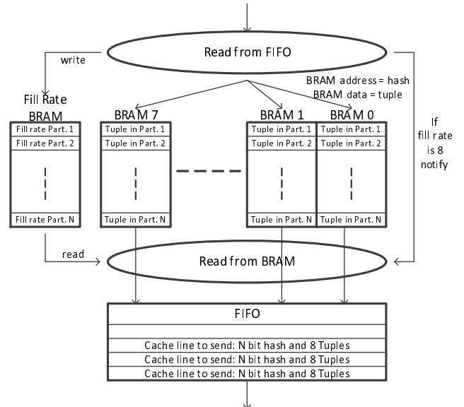
Figure 6: Design of the write combiner module for 8B tuples.
