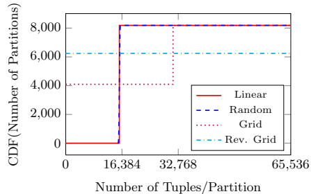
(a) Radix partitioning is applied.
