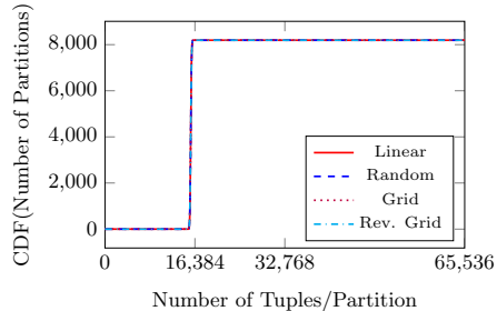
(b) Hash partitioning is applied.
